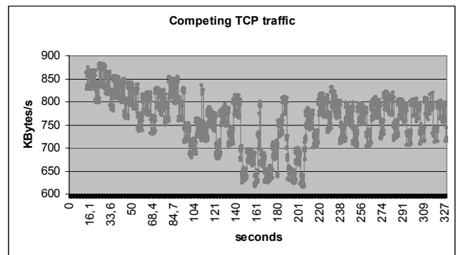
Figure 7. TCP traffic
